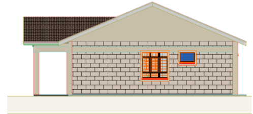
SOUTH ELEVATION 1:100
