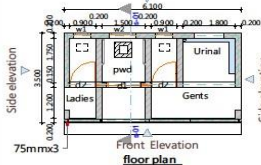
floor plan
