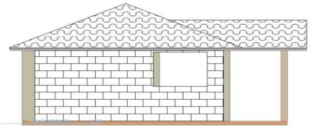
ELEVATION 03
