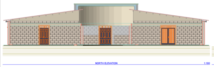
NORTH ELEVATION 1:100
