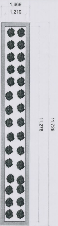
PROPAGATOR PLAN LAYOUT SCALE 1:100
