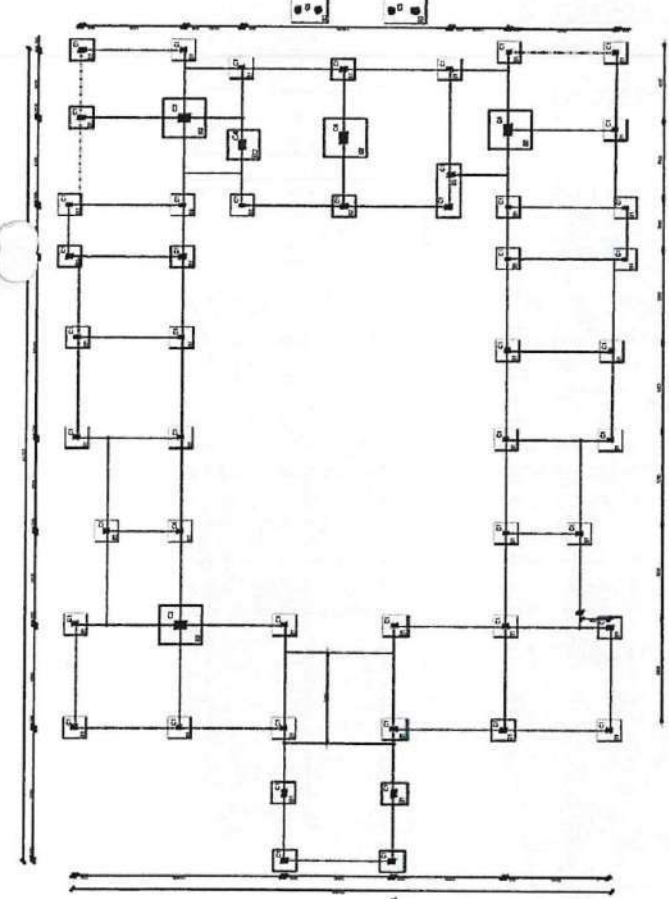
FOUNDATION LAYOUT
